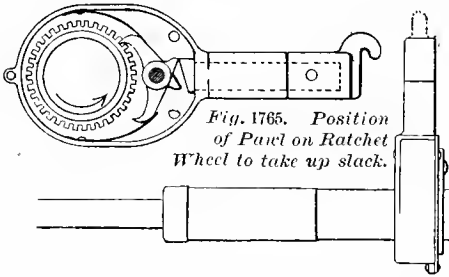
THE HINCKLEY BRAKE SLACK ADJUSTER EQUIPMENT C.
